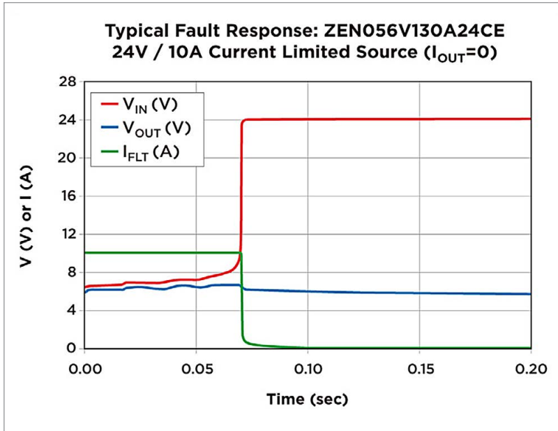
Figure 2: Typical fault response of a PolyZen device
