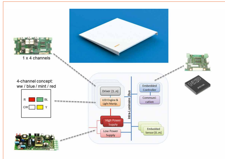
Figure 5: “Wedge” luminaire and luminaire architecture
