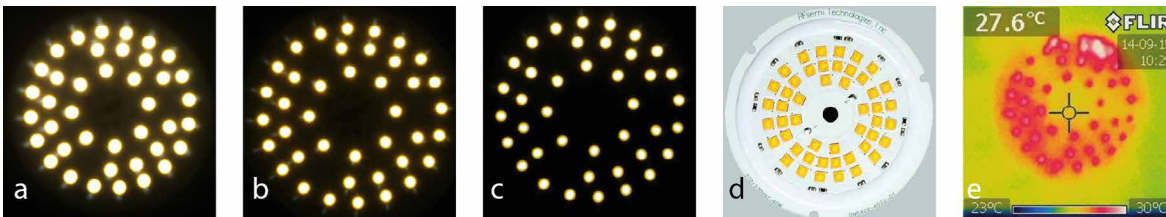
Figures 2 a-e: The EL01 LED modules dimmed to 5 W (a), dimmed to 2 W (b), dimmed to 1 W (c), chips are mounted all around the edge (d), leading to an even thermal distribution (e). Many other AC concepts use a sequential dimming concept with just one central IC
