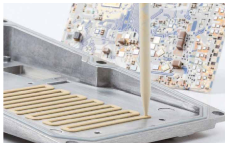
The heat-conducting SEMICOSIL® 961 TC silicone filler from Wacker is applied directly to the heat sink. Once the electrical circuit is pressed on, the gap filler cures to form a soft, cushioning silicone layer that optimally transfers heat to the heat sink
