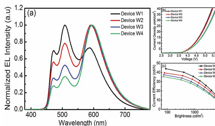
(a) EL spectra of the devices based on different thicknesses of Ir(MDQ)2(acac) varying from 0.02 nm (W1), 0.04 nm (W2), 0.06 nm (W3) and 0.08 nm (W4), (b) J-V curves, and (c) Current efficiency–brightness characteristics of the devices
