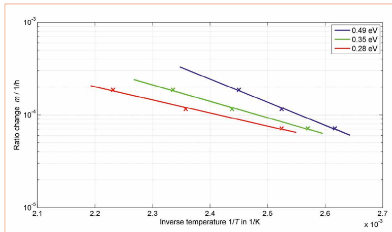
Figure 6: Arrhenius graphs for an LED package (LED type A) for different temperatures
