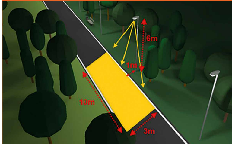
Figure 5: Schematic view of the street lighting setup with 10 m pole spacing, 6 m pole height, 1 m distance away from the road. The yellow rectangle shows the area to be illuminated [1]
