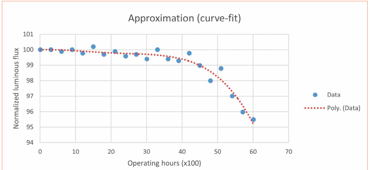
Figure 3: Lumen output over time with curve-fit through the average values
