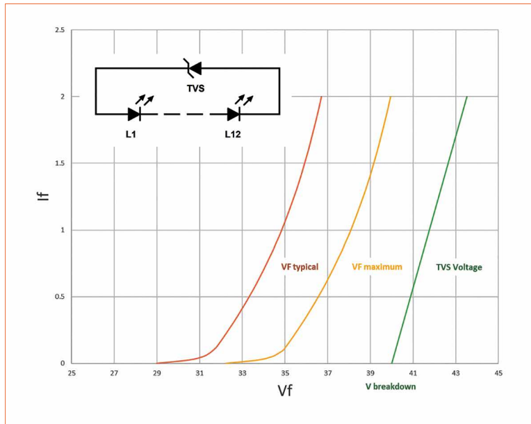
Figure 6: Badly designed Transient Voltage Suppressor that never protects the LED as it does not cross the LED curves
