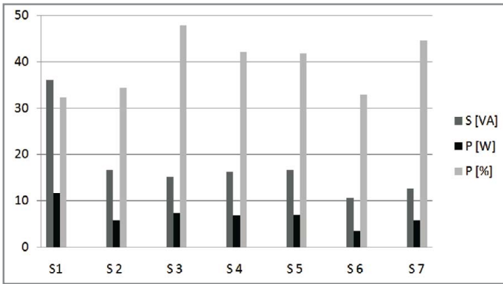
Figure 3: Mains power values of the tested LED bulbs. X-axis: S1 to S7 showing numbers of the tested samples. Y-axis: Apparent power level S in VA (dark grey bars), active power level in W (black bars) and the relation of the active power to the apparent power in percentage (light grey bars).
