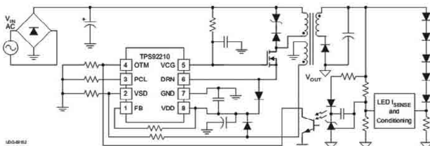
Functional diagram using TI's new TPS92210 LED driver
