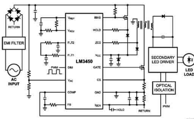
A typical application circuit using the LM3450
