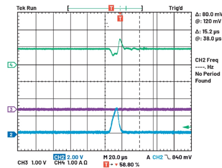
Figure 4: The MAX25608 LED short detection (Channel 2: Drain voltage; Channel 3: FLTb; Channel 4: LED current).
