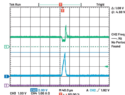
Figure 3: The MAX25608 LED open detection (Channel 2: Drain voltage; Channel 3: FLTb; Channel 4: LED current).
