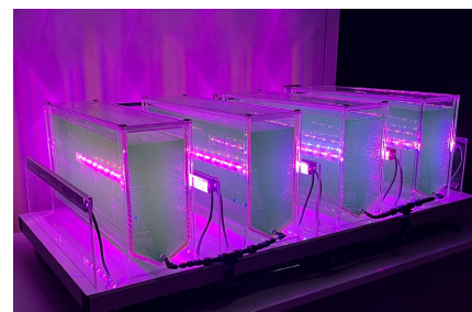
Pilot plant for microalgae cultivation.
